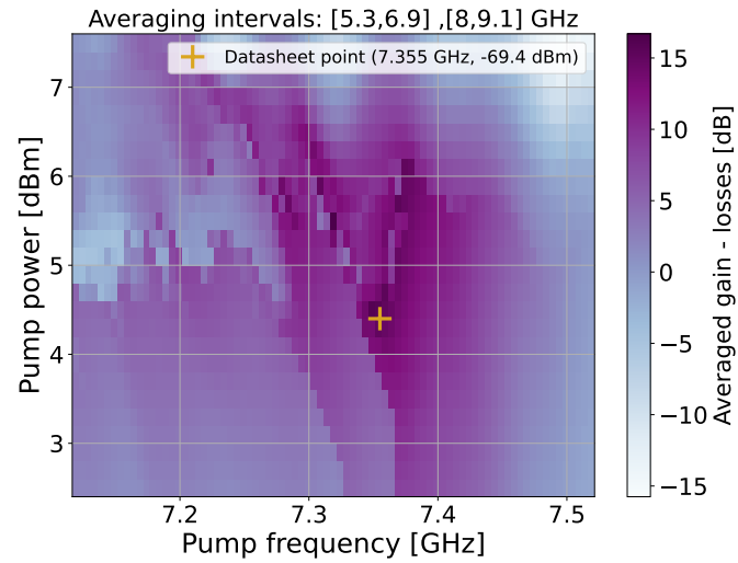
Figure 8: Averaged gain of the TWPA referred to a through line as a function of the pump frequency and the pump power (at the output of the pump source). The operating point used for the other figures in the datasheet is indicated by the yellow marker (with the pump power specified at the input of the TWPA).
