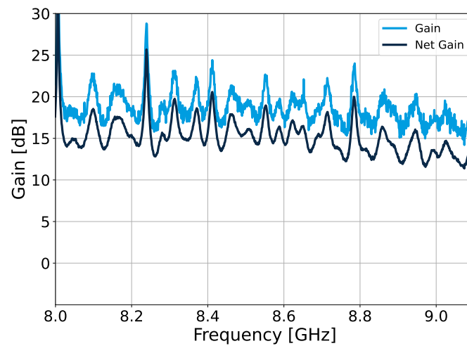
Figure 4: Zoom on the gain (ON-OFF) and net gain (ON-lossless reference) of the TWPA. The pump parameters are (at the input of the TWPA): 7.355 GHz and -69.4 dBm.
