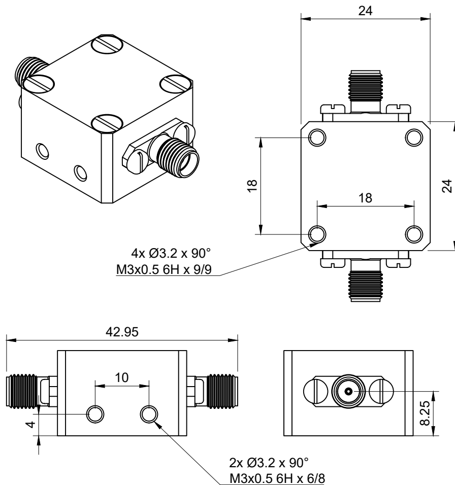
Figure 9: Schematic of the box
