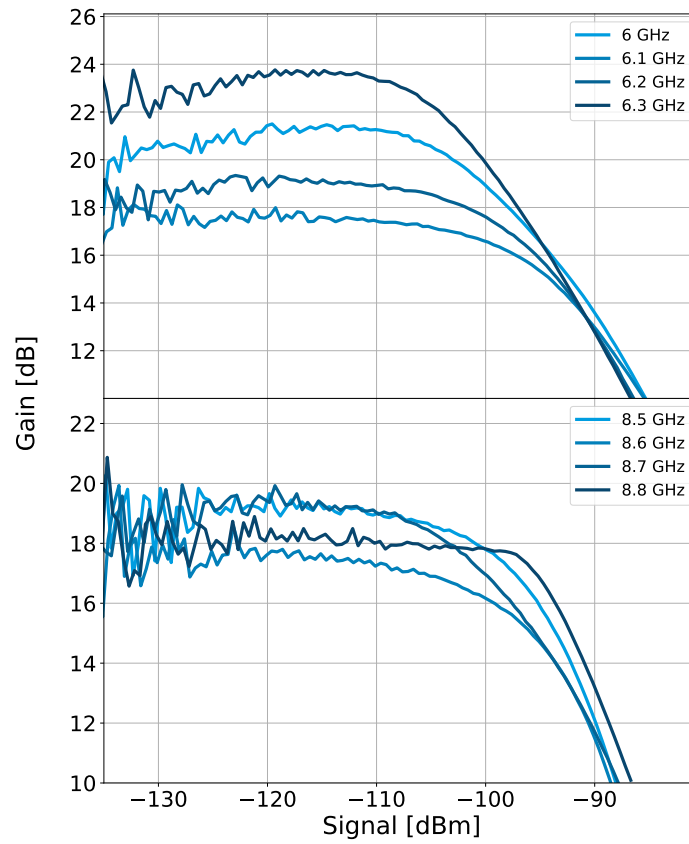
Figure 5: Graph of several saturation curves. The signal power corresponds to the signal at the input of the TWPA.
