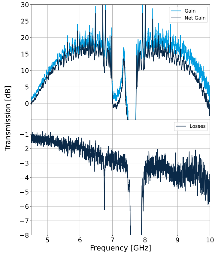
Figure 2: Top panel shows the gain (ON-OFF) and net gain (ON-lossless reference) of the TWPA. The pump parameters are (at the input of the TWPA): 7.355 GHz and -69.4 dBm. Bottom panel shows the electrical losses within the TWPA. The gap is centered at 7.71 GHz and is 0.46 GHz wide, the signal cannot propagate in the gap.
