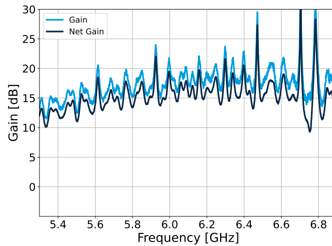
Figure 3: Zoom on the gain (ON-OFF) and net gain (ON-lossless reference) of the TWPA. The pump parameters are (at the input of the TWPA): 7.355 GHz and -69.4 dBm.
